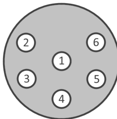
Connector: MCBH-6F-TI, External View
